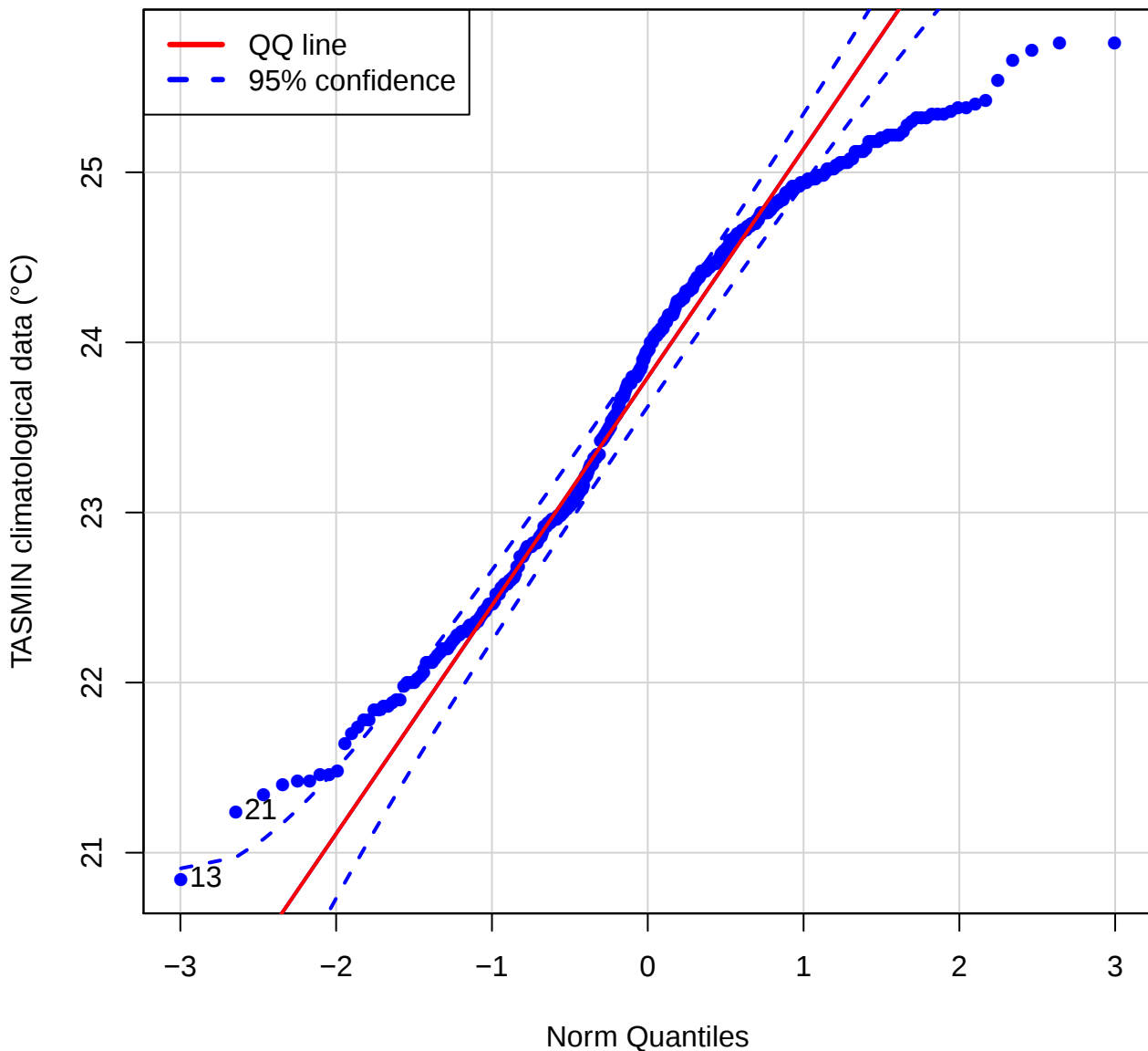
QQ plot (TASMIN of STLC)
