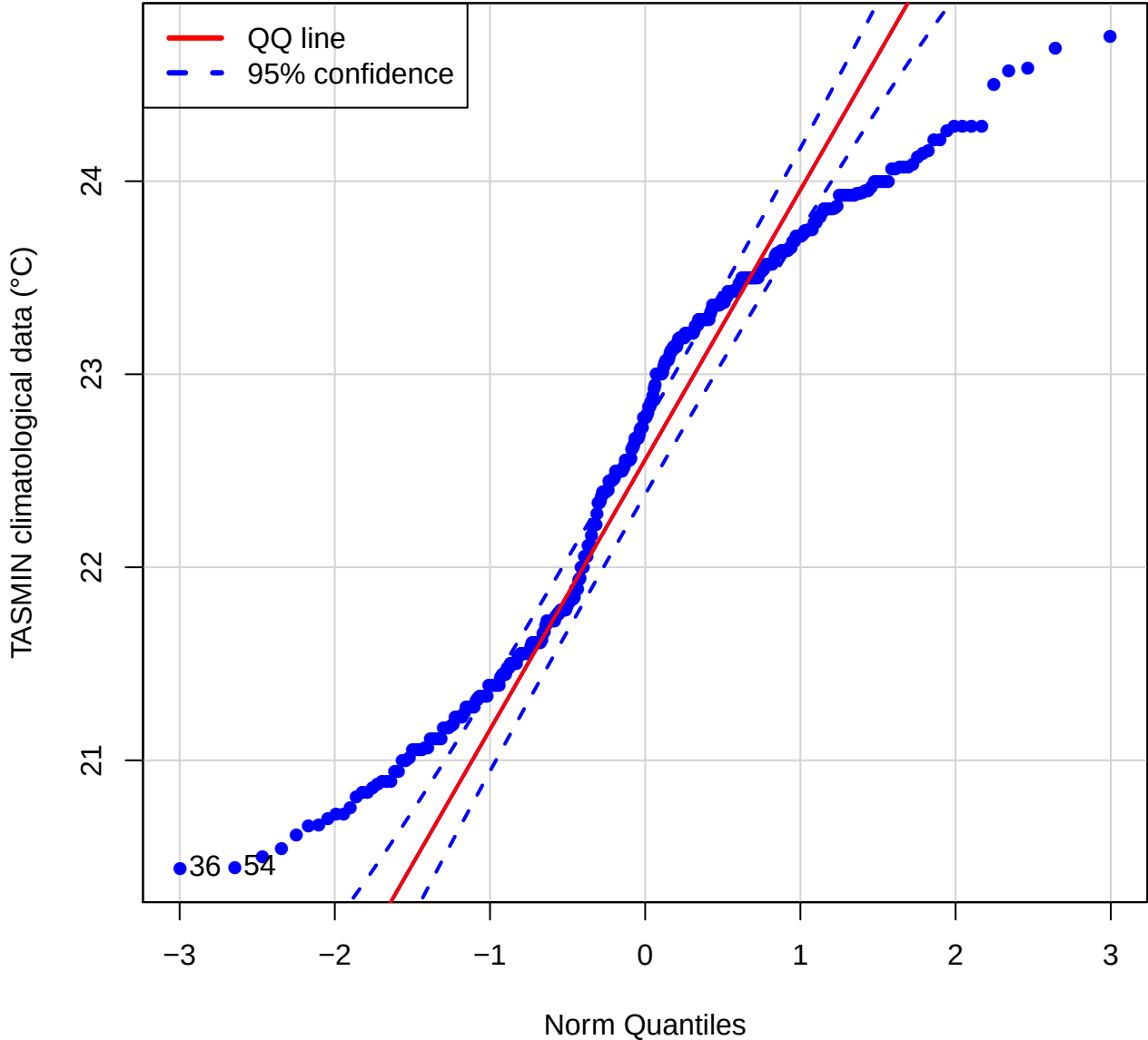
QQ plot (TASMIN of STMB)
