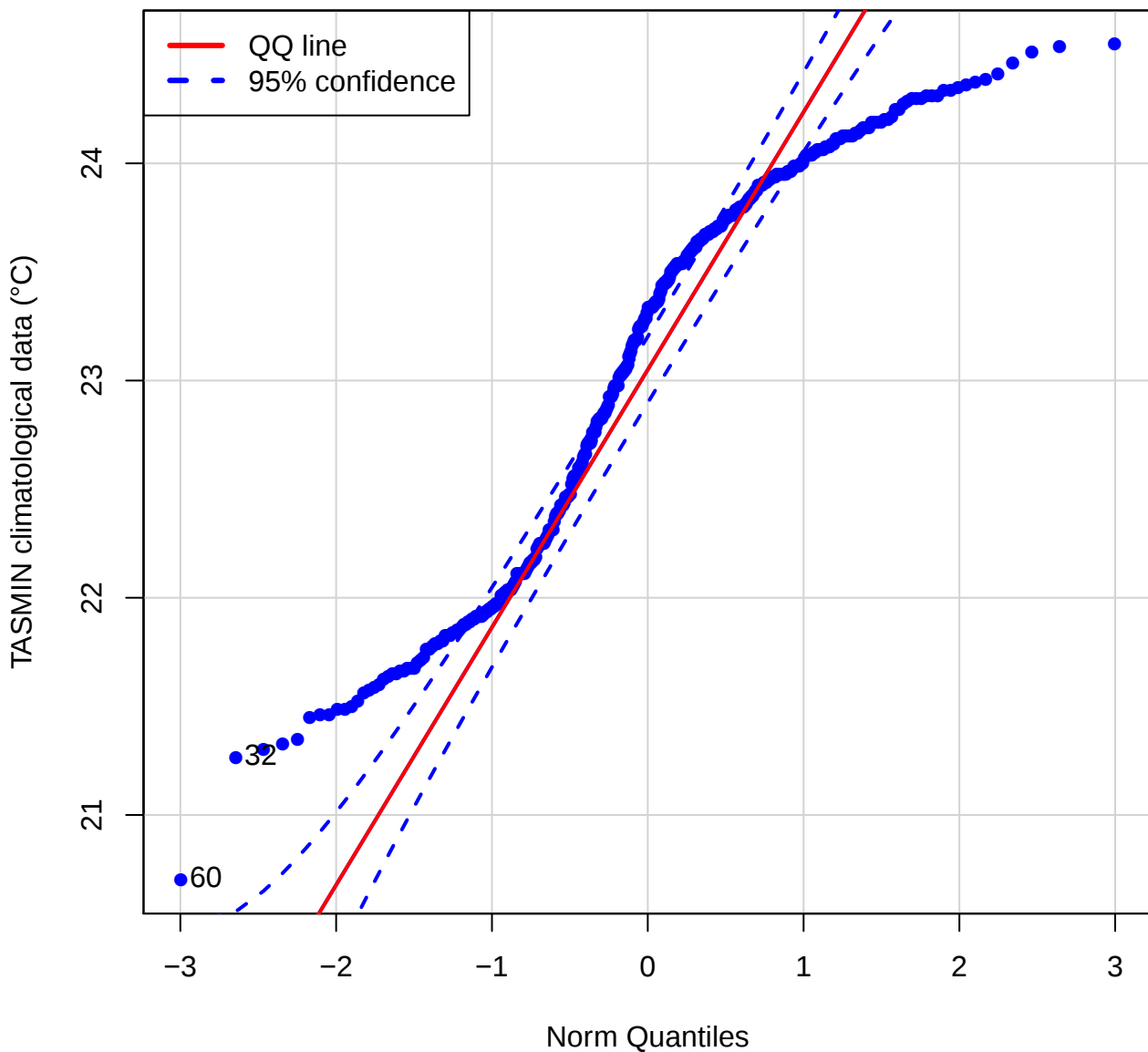
QQ plot (TASMIN of STMC)
