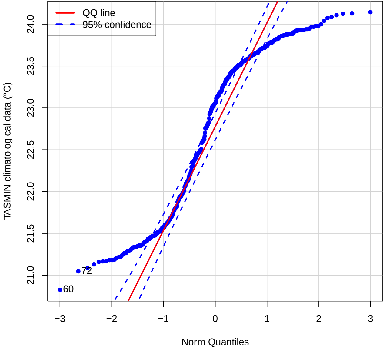
QQ plot (TASMIN of STMP)
