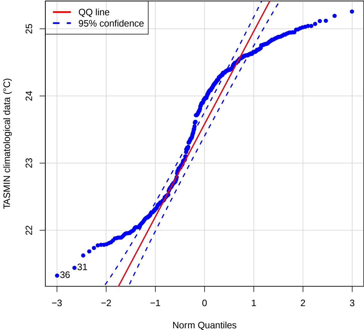
QQ plot (TASMIN of STPR)
