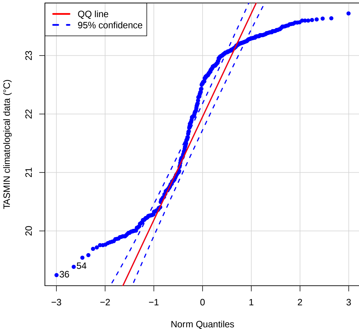
QQ plot (TASMIN of TILP)
