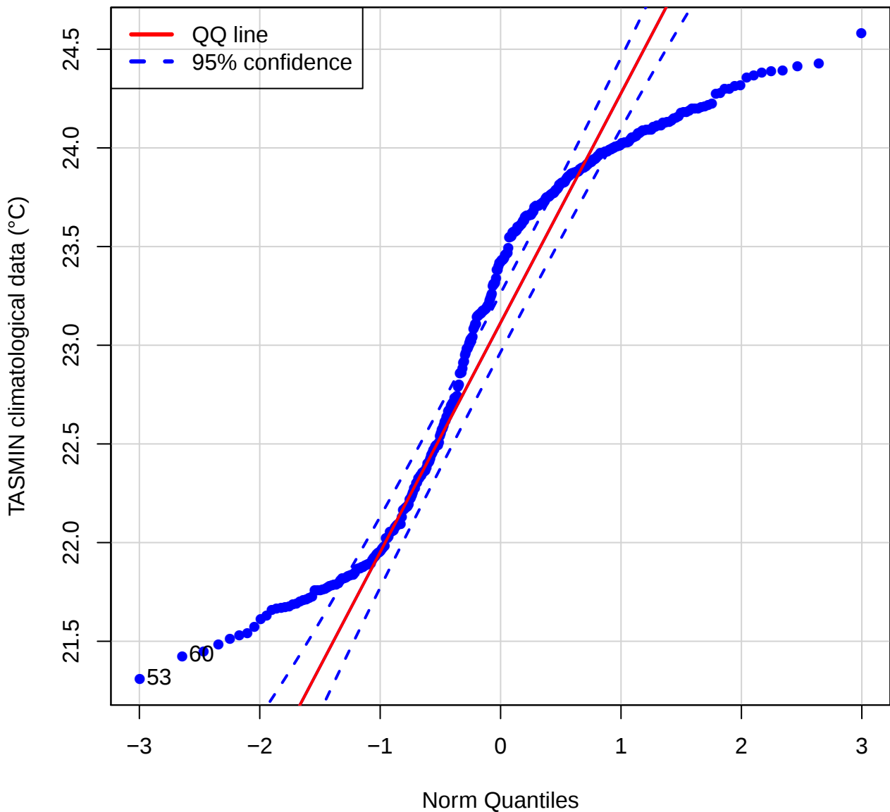
QQ plot (TASMIN of VCLR)
