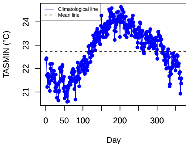
Climatology (BASP)
