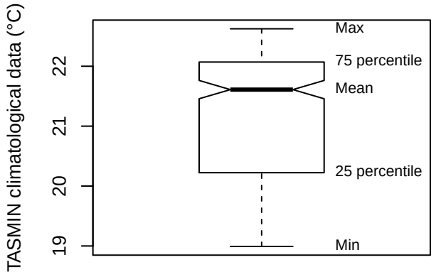
Box plot (BLLF)
