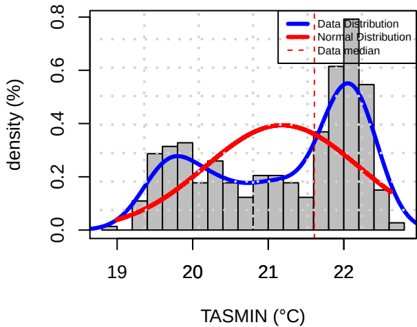
Histogram Distribution (BLLF)
