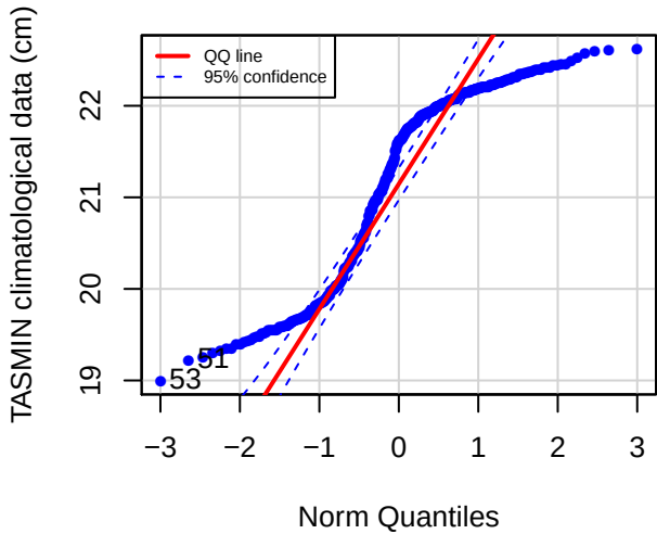
QQ plot (BLLF)
