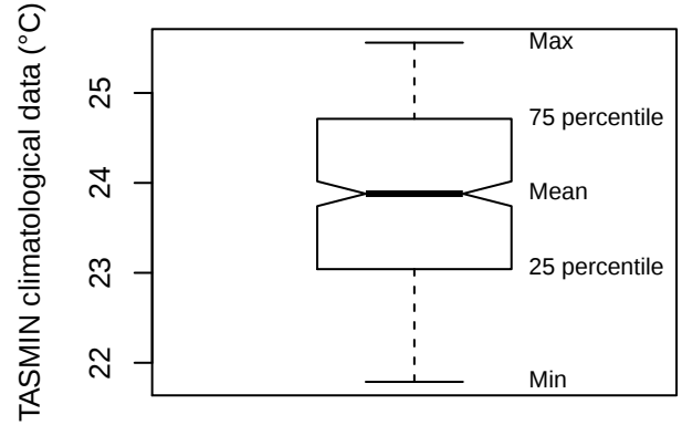
Box plot (DUCO)
