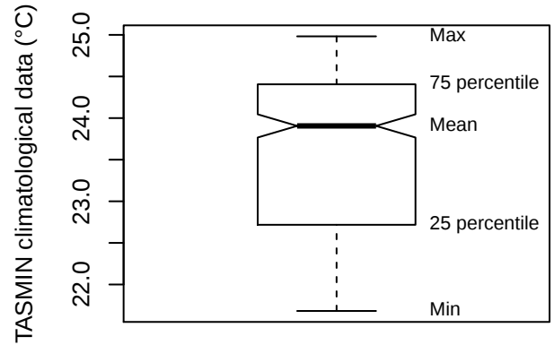
Box plot (FDFD)
