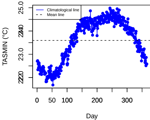
Climatology (FDFD)
