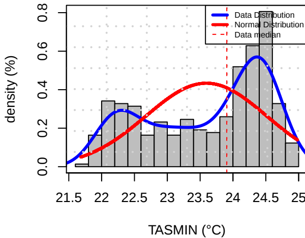
Histogram Distribution (FDFD)
