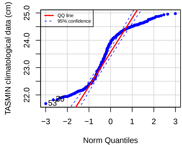
QQ plot (FDFD)
