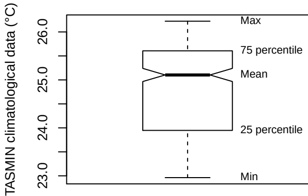
Box plot (FDFD)
