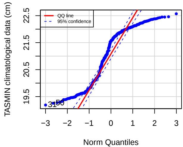
QQ plot (FSDC)
