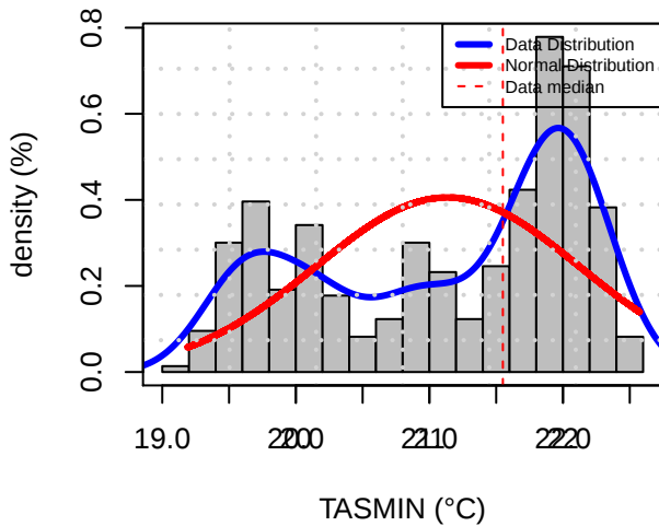
Histogram Distribution (FSDC)
