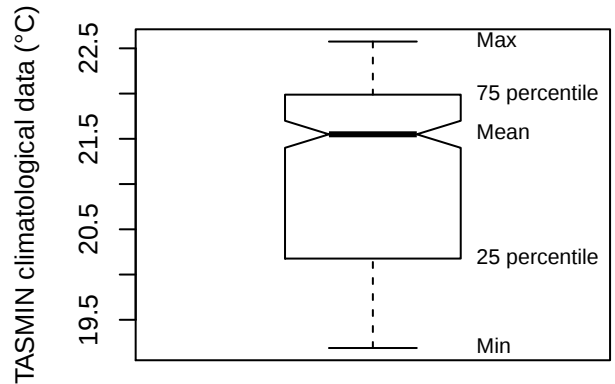
Box plot (FSDC)
