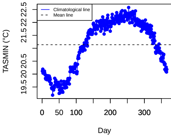
Climatology (FSDC)
