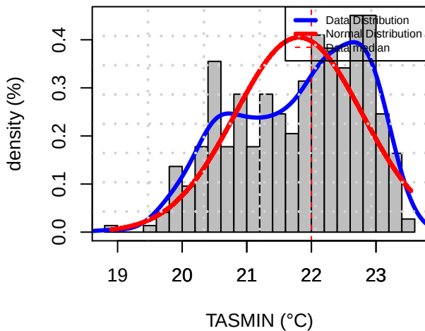
Histogram Distribution (FSDG)
