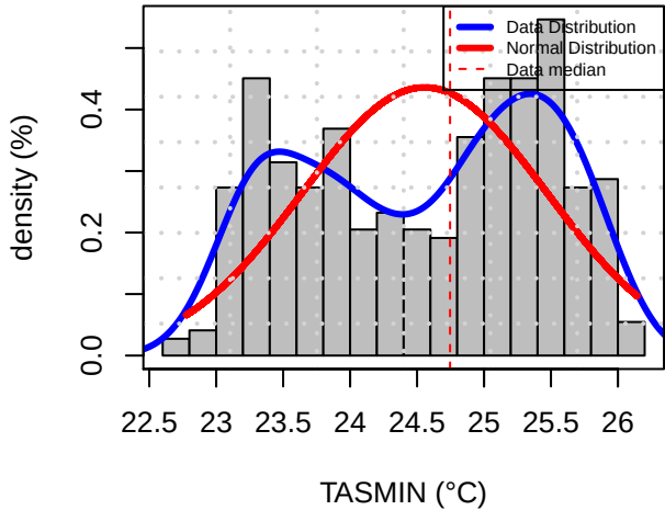
Histogram Distribution (GDRV)
