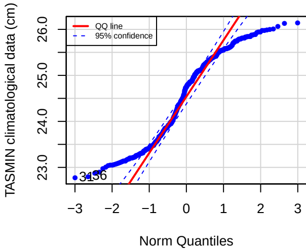
QQ plot (GDRV)
