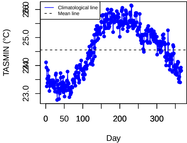
Climatology (GDRV)
