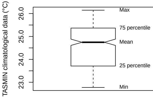
Box plot (GDRV)
