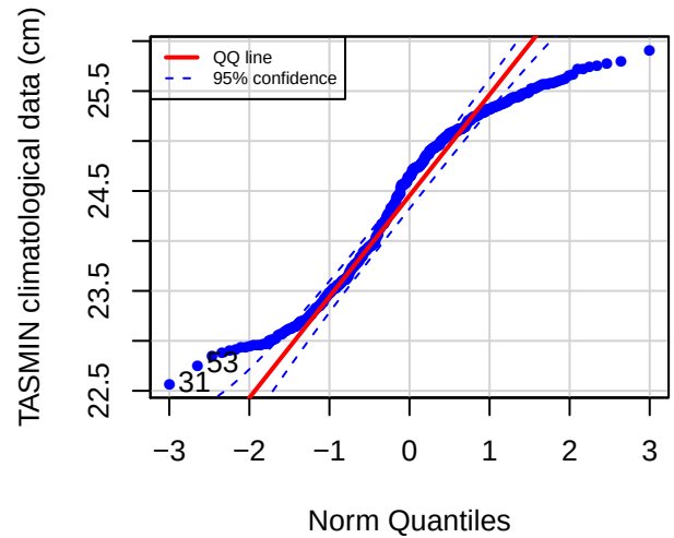
QQ plot (LFRC)
