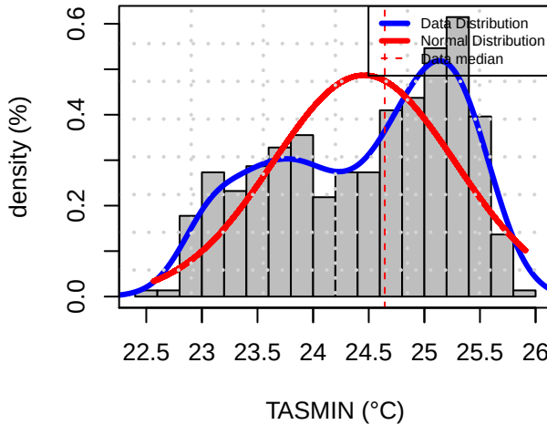
Histogram Distribution (LFRC)
