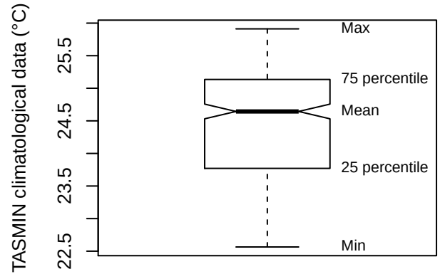
Box plot (LFRC)
