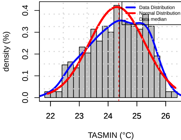
Histogram Distribution (LFRS)
