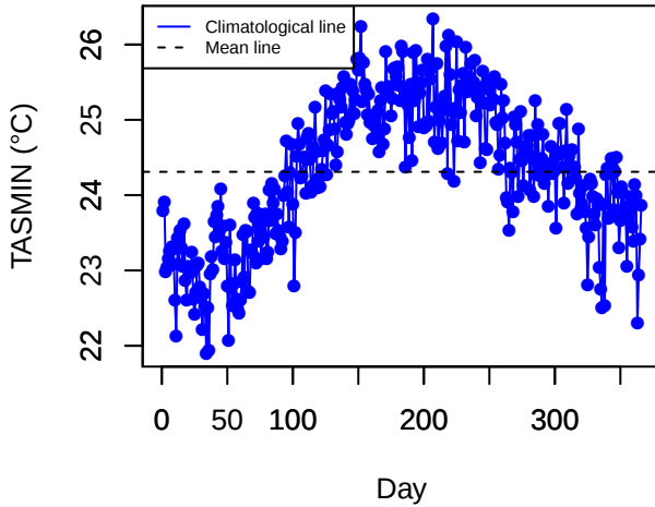
Climatology (LFRS)
