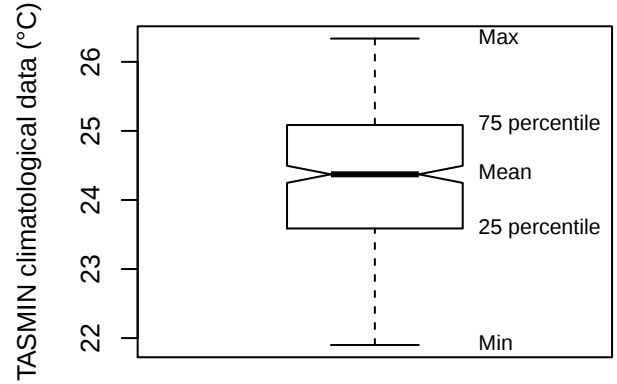
Box plot (LFRS)
