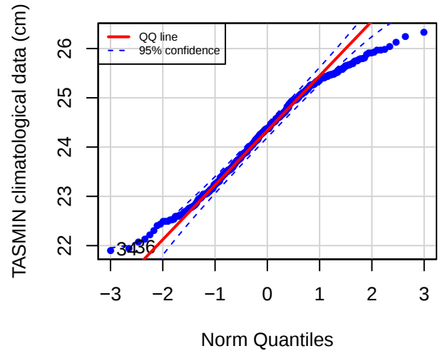
QQ plot (LFRS)
