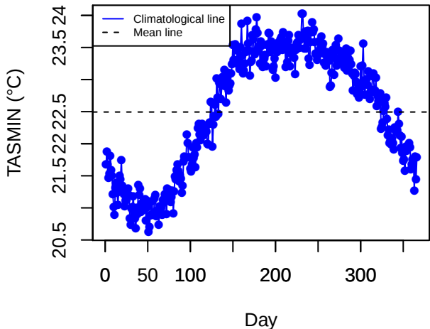
Climatology (MACB)
