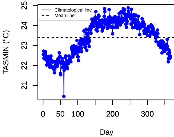
Climatology (MARB)
