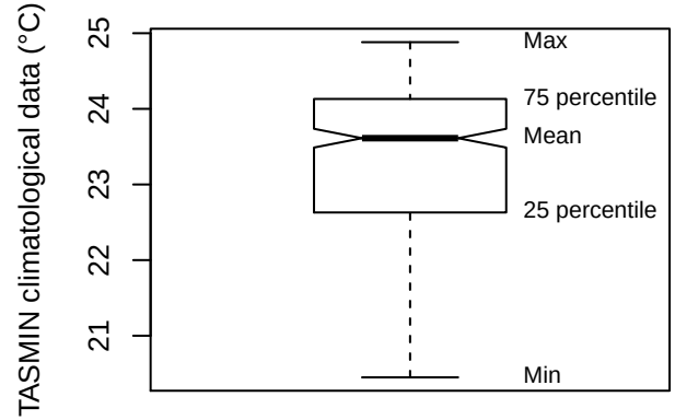
Box plot (MARB)
