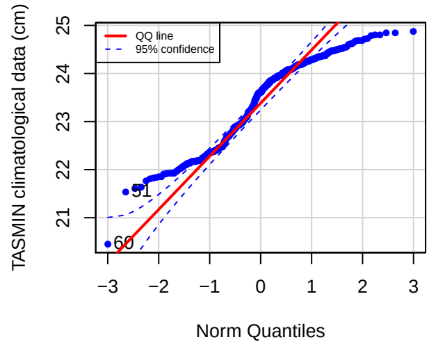
QQ plot (MARB)
