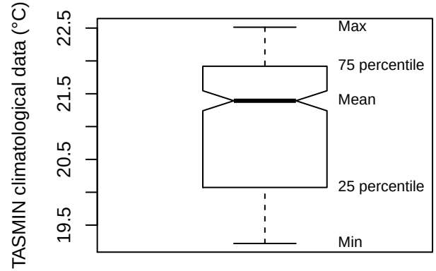
Box plot (MRRD)
