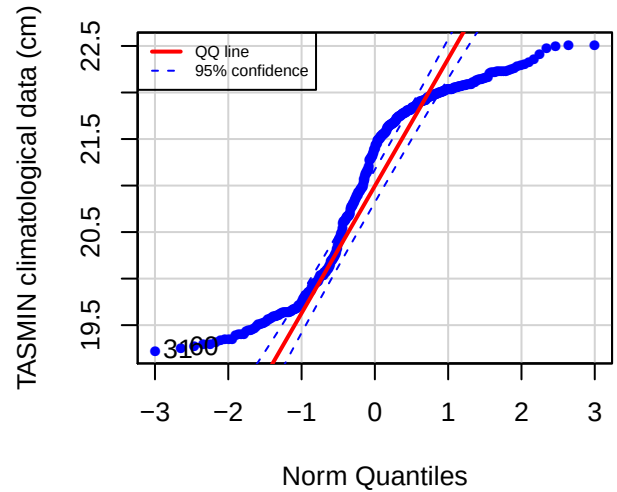
QQ plot (MRRD)
