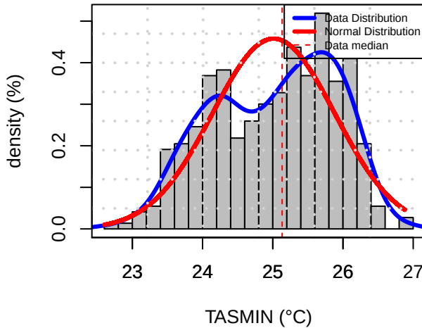
Histogram Distribution (PANS)
