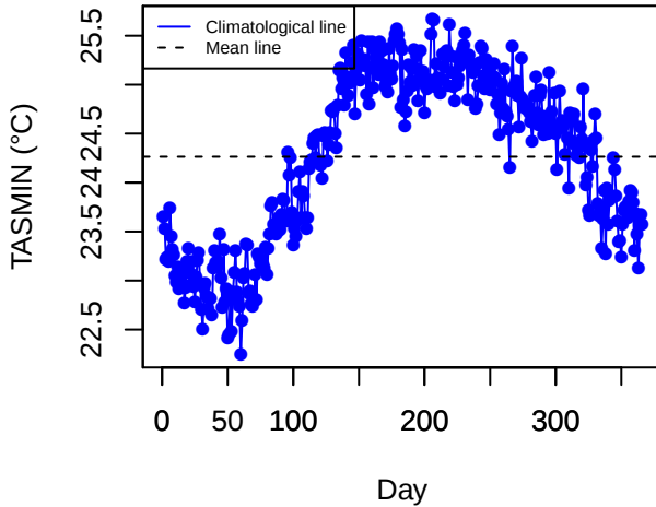
Climatology (RVPE)
