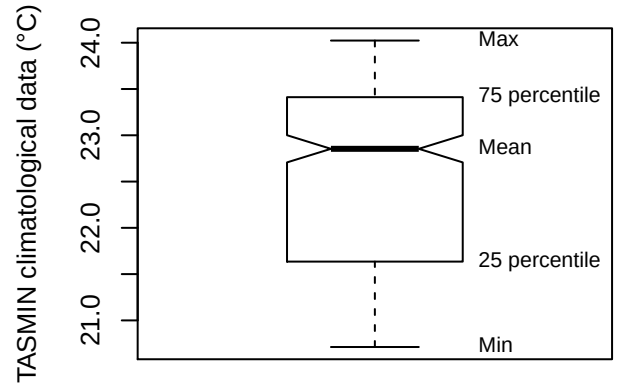
Box plot (STJO)
