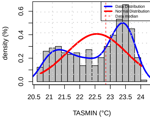
Histogram Distribution (STJO)
