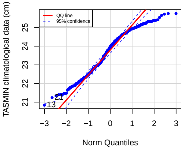
QQ plot (STLC)
