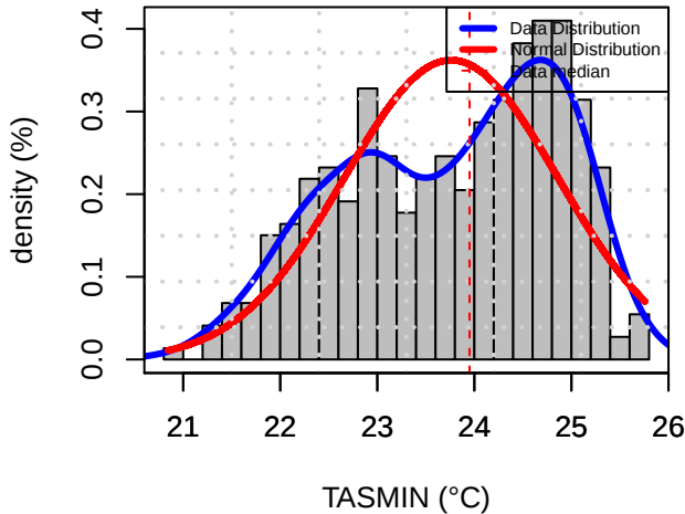
Histogram Distribution (STLC)
