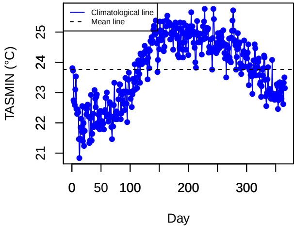
Climatology (STLC)
