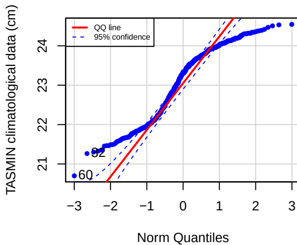
QQ plot (STMC)
