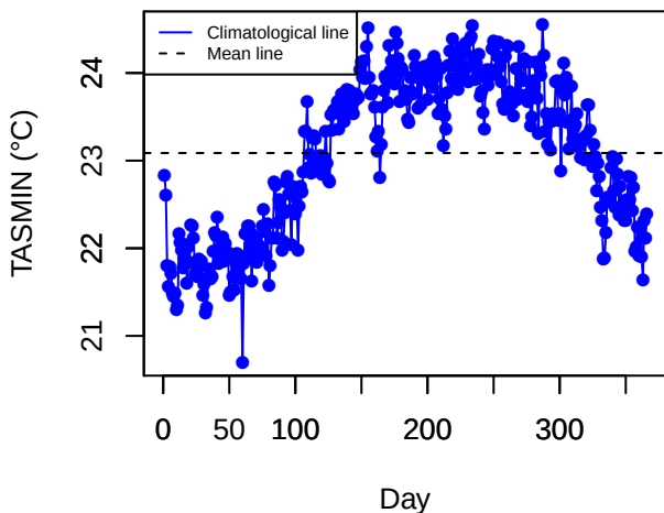
Climatology (STMC)
