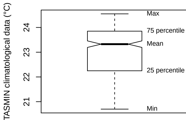
Box plot (STMC)
