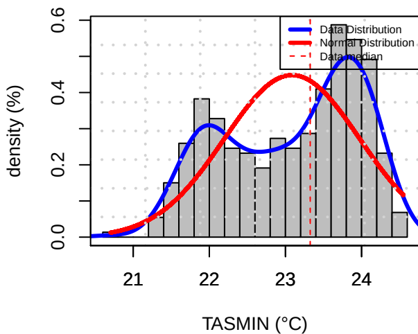
Histogram Distribution (STMC)
