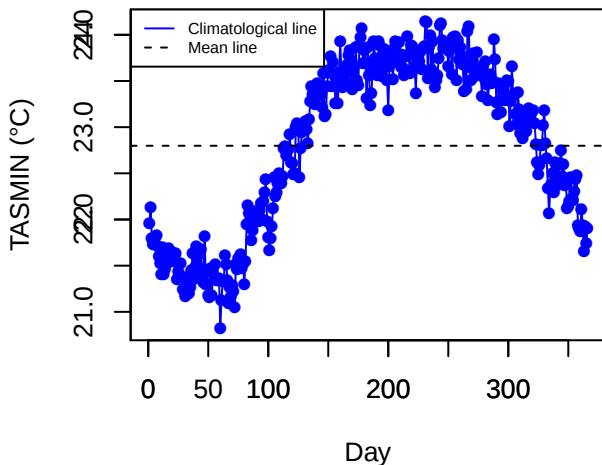
Climatology (STMP)
