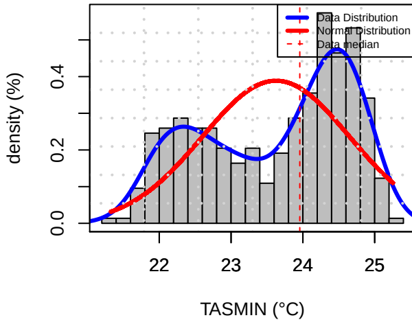
Histogram Distribution (STPR)
