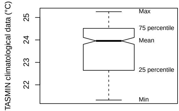
Box plot (STPR)
