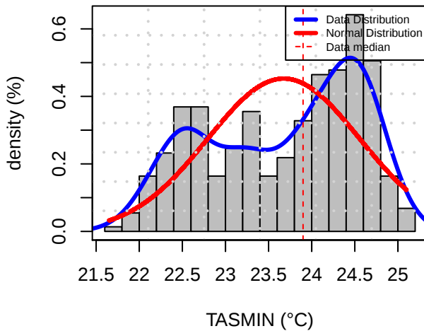
Histogram Distribution (TRTR)
