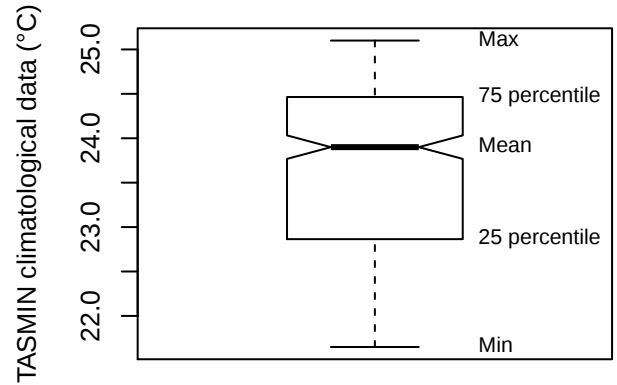
Box plot (TRTR)
