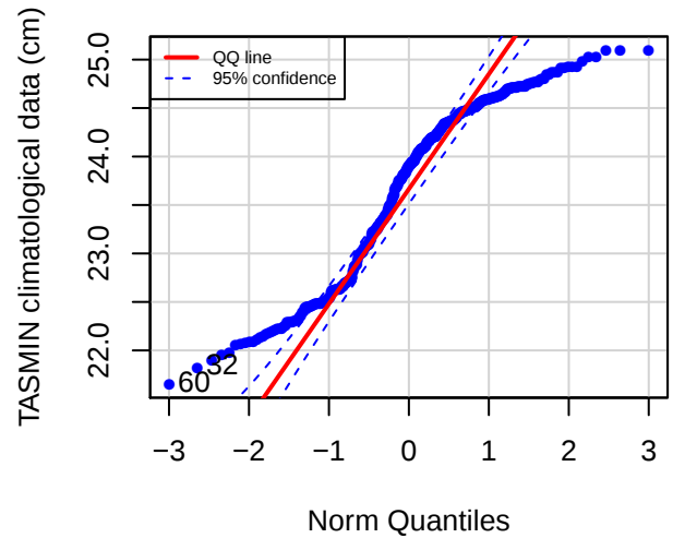
QQ plot (TRTR)
