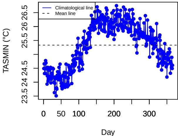
Climatology (VCLC)
