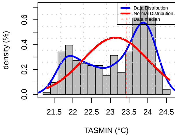
Histogram Distribution (VCLR)
