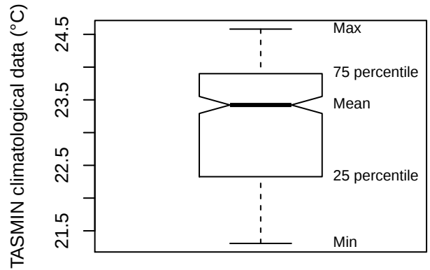
Box plot (VCLR)
