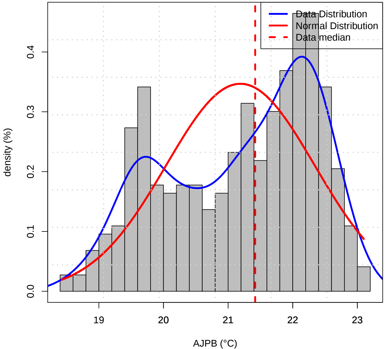
Histogram of Data distribution (TASMIN of AJPB)
