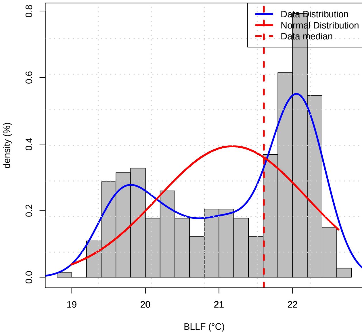
Histogram of Data distribution (TASMIN of BLLF)
