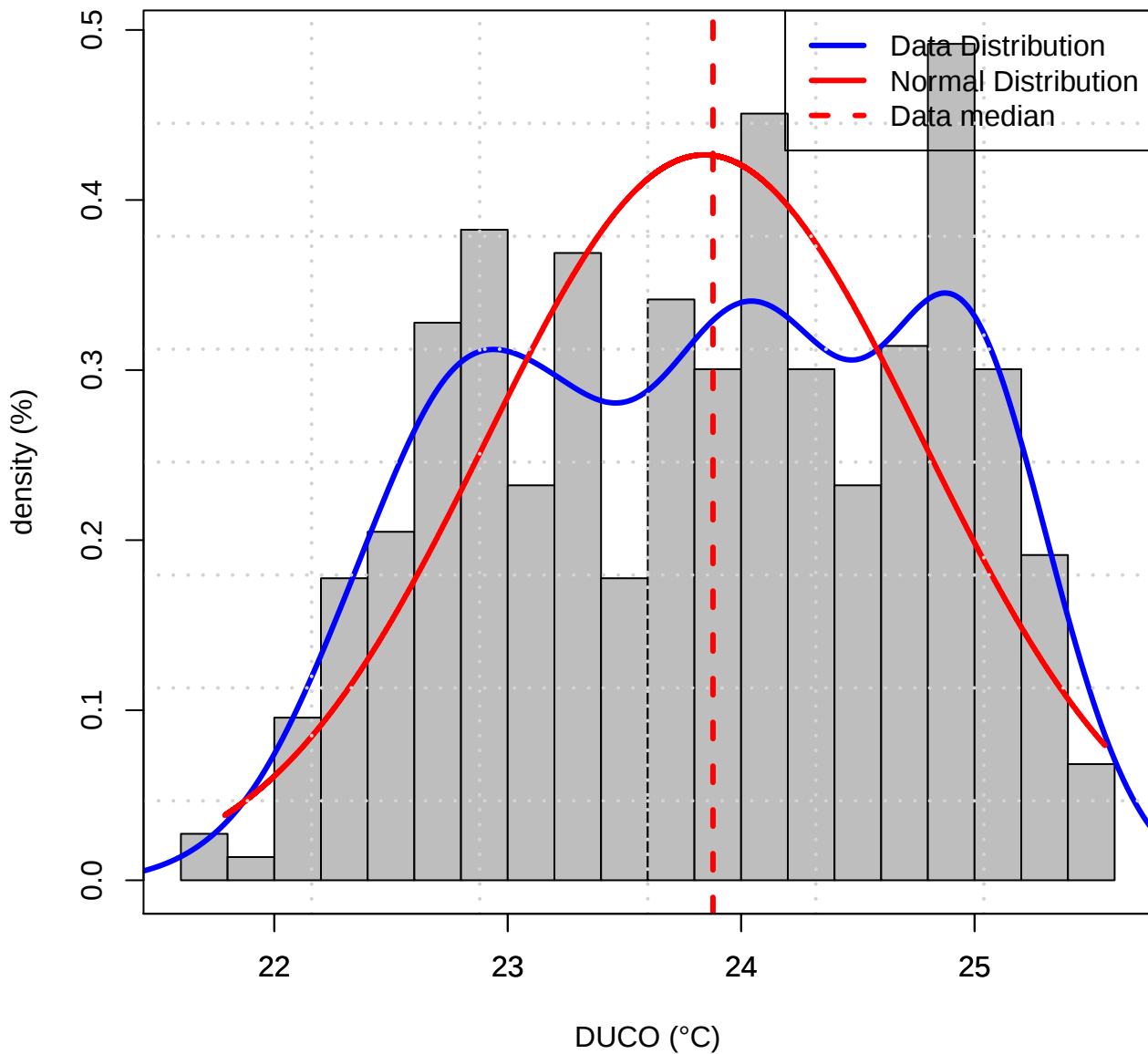
Histogram of Data distribution (TASMIN of DUCO)
