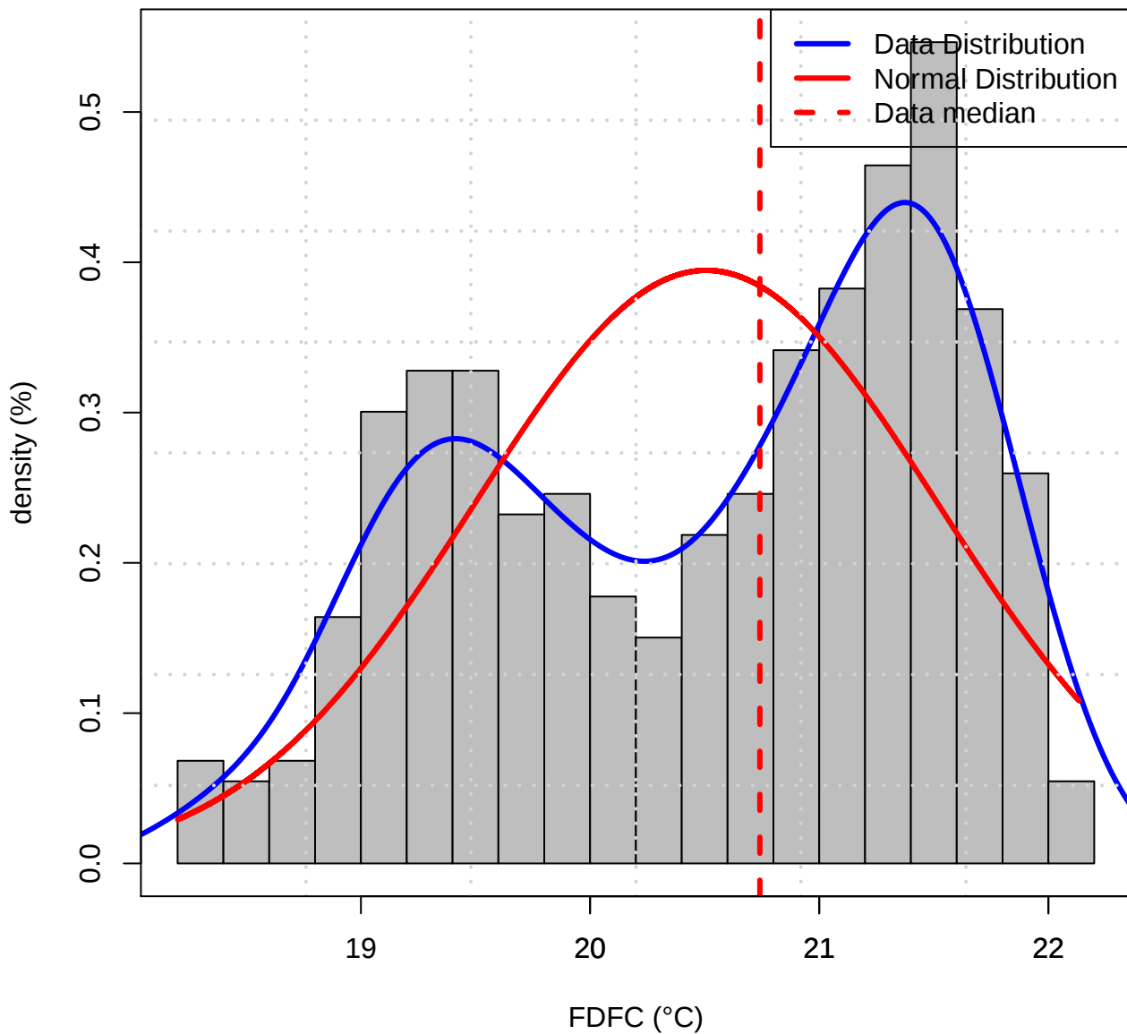
Histogram of Data distribution (TASMIN of FDFC)
