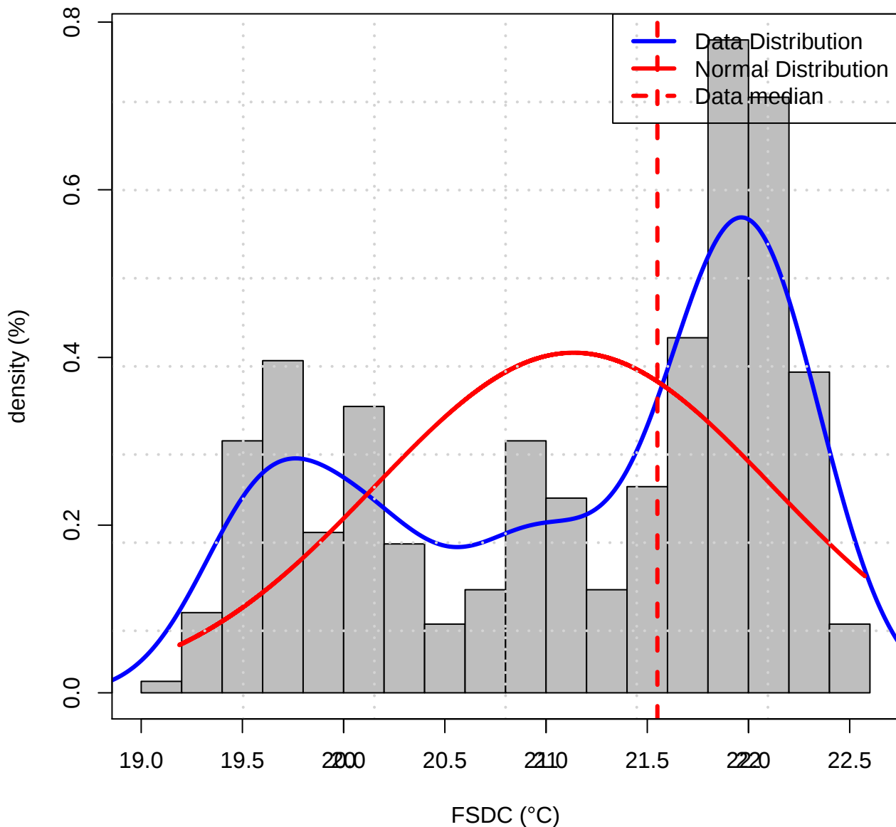
Histogram of Data distribution (TASMIN of FSDC)
