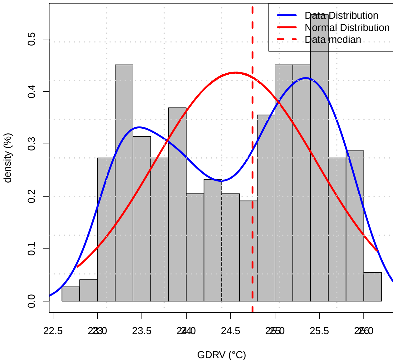
Histogram of Data distribution (TASMIN of GDRV)
