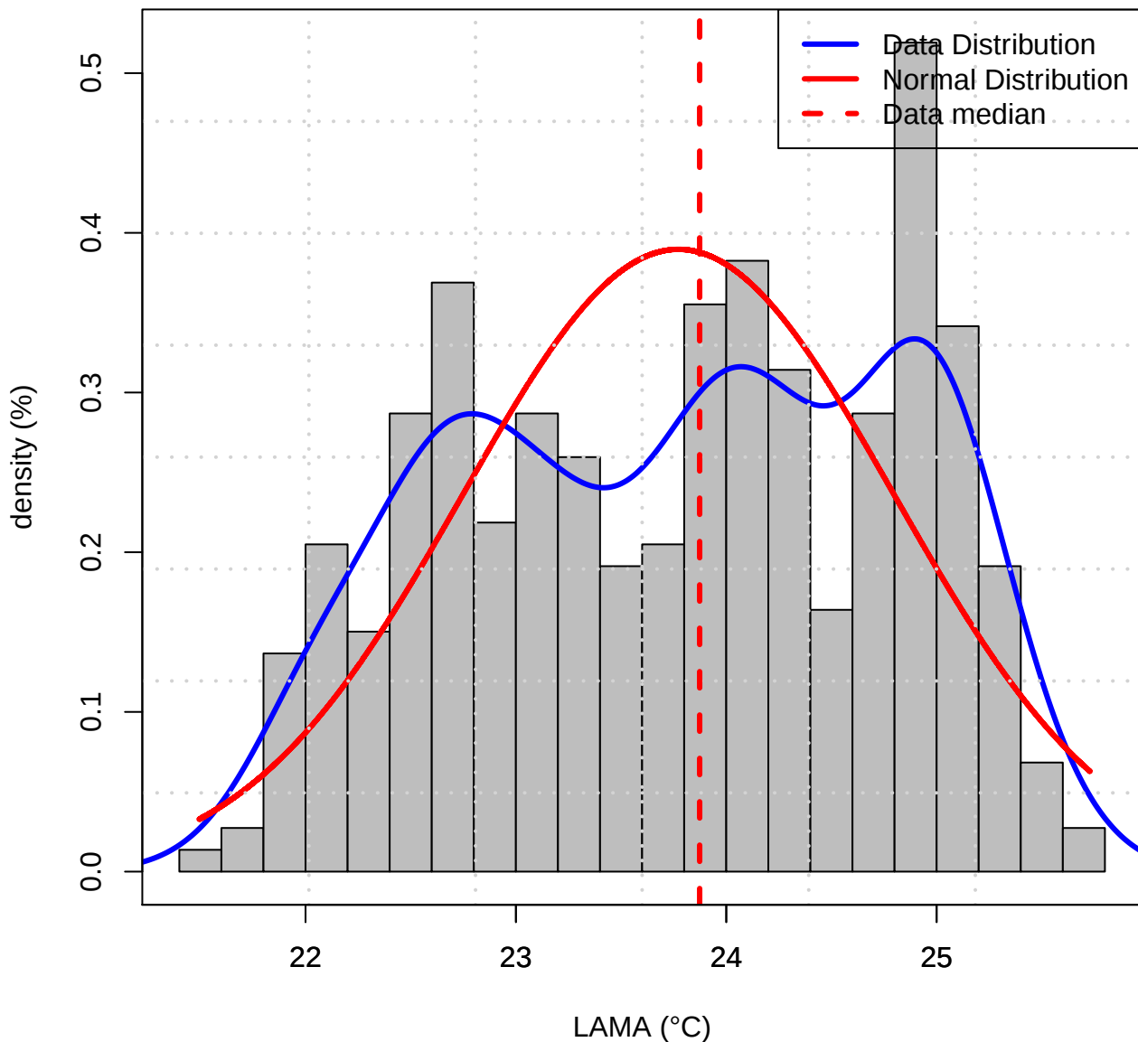
Histogram of Data distribution (TASMIN of LAMA)
