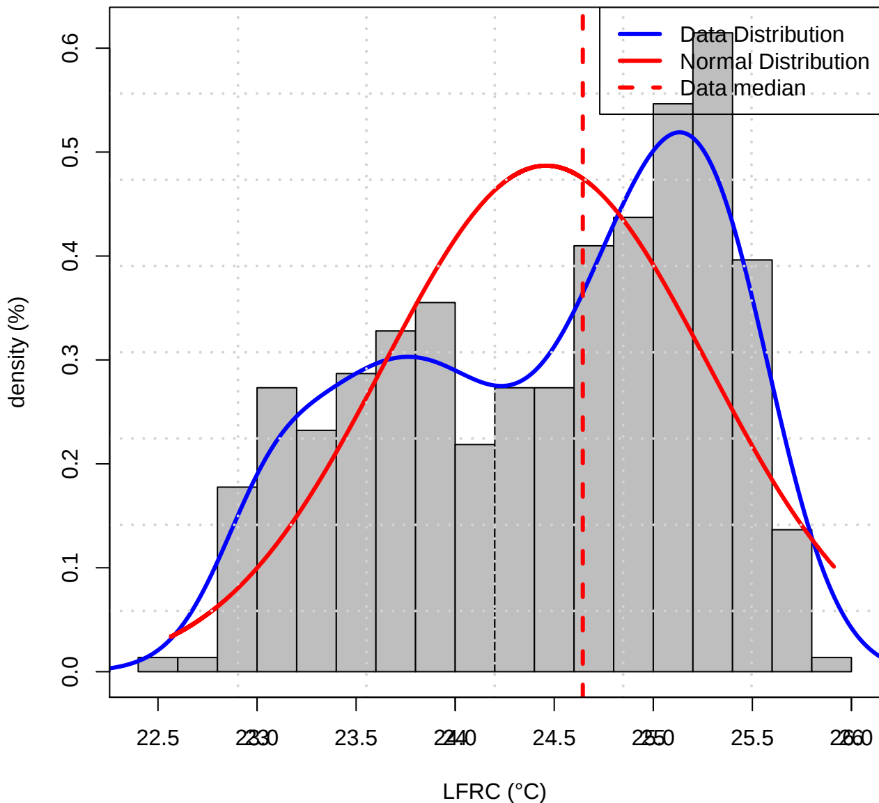
Histogram of Data distribution (TASMIN of LFRC)
