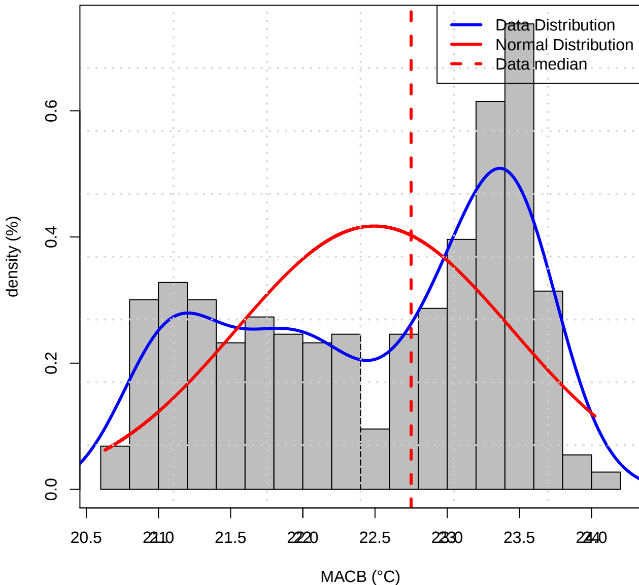
Histogram of Data distribution (TASMIN of MACB)
