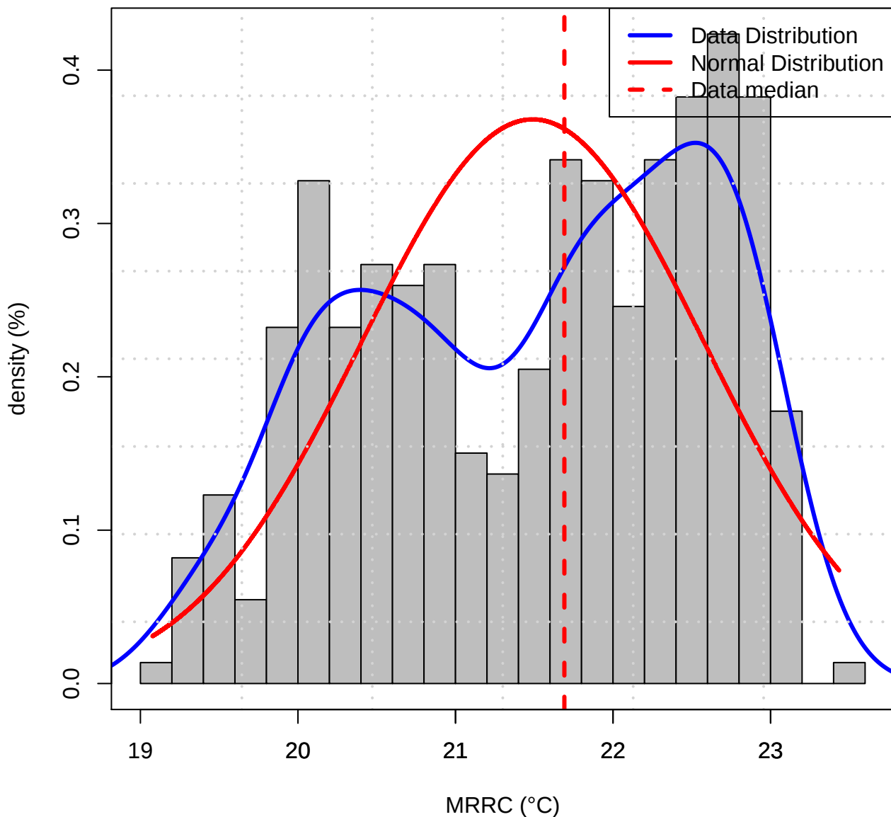
Histogram of Data distribution (TASMIN of MRRC)
