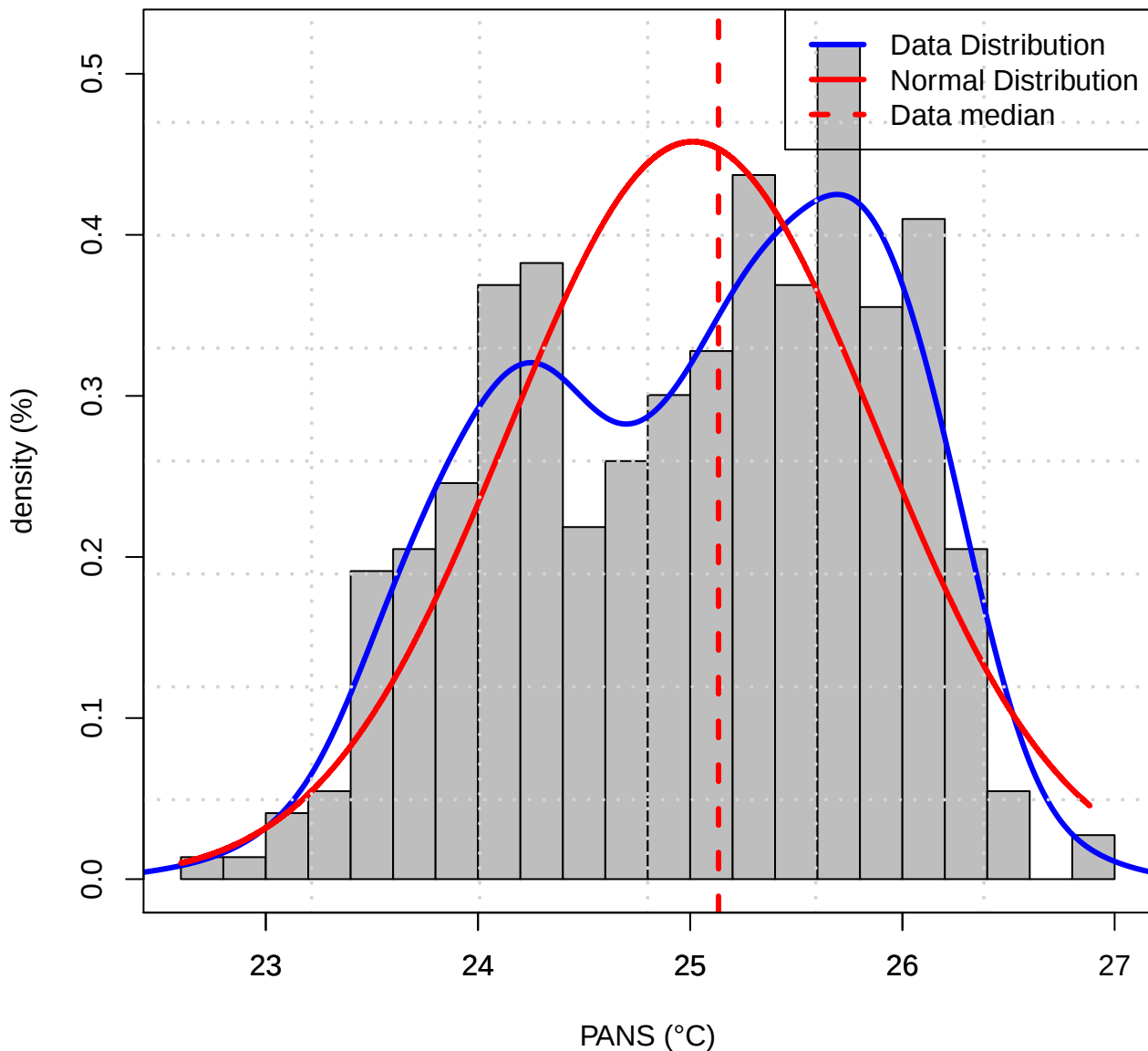
Histogram of Data distribution (TASMIN of PANS)
