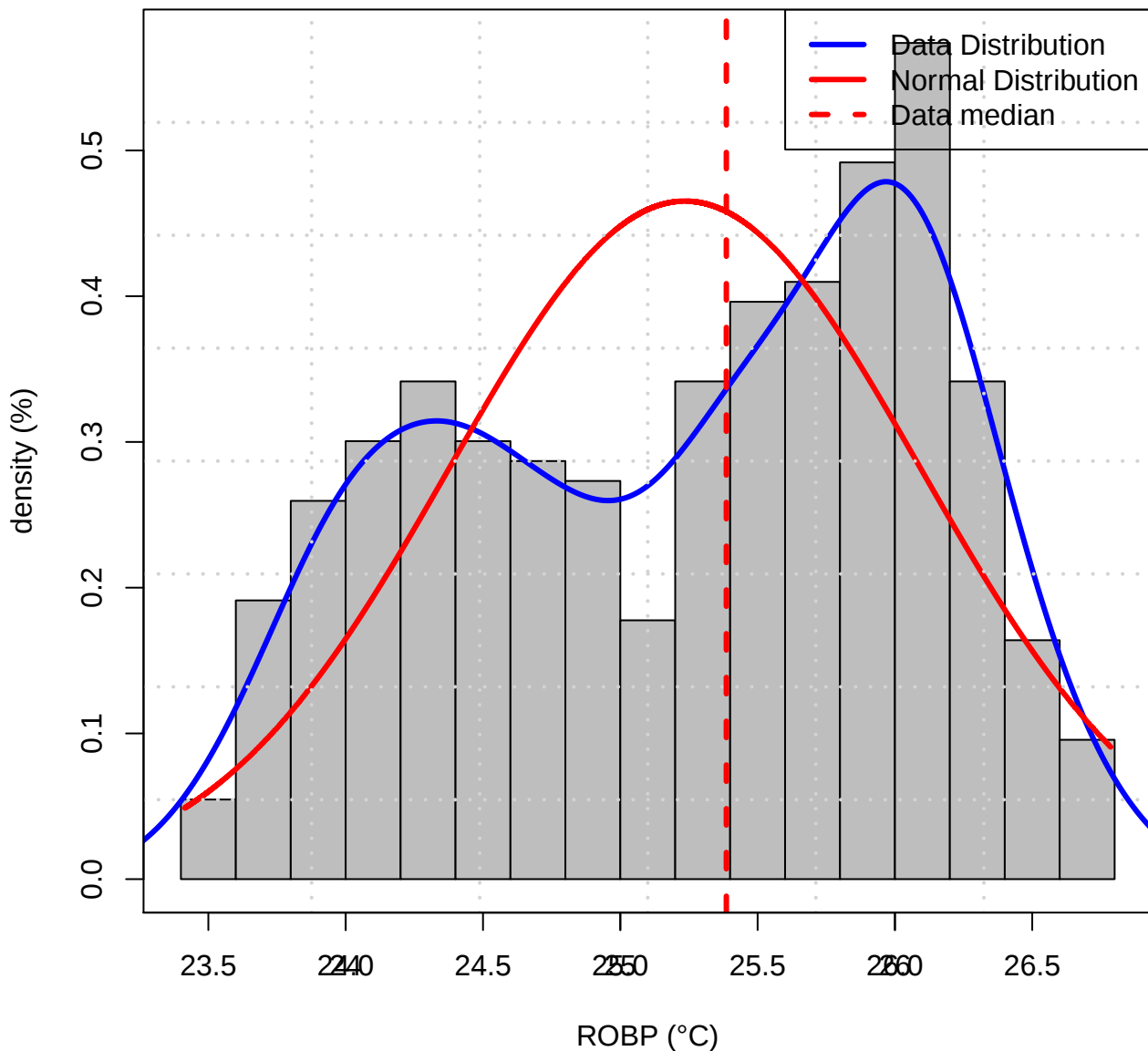
Histogram of Data distribution (TASMIN of ROBP)
