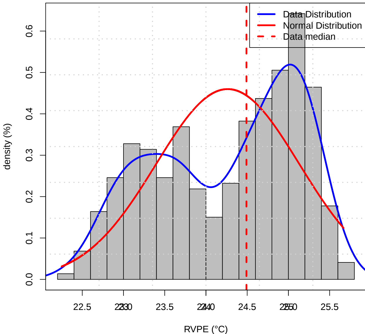
Histogram of Data distribution (TASMIN of RVPE)
