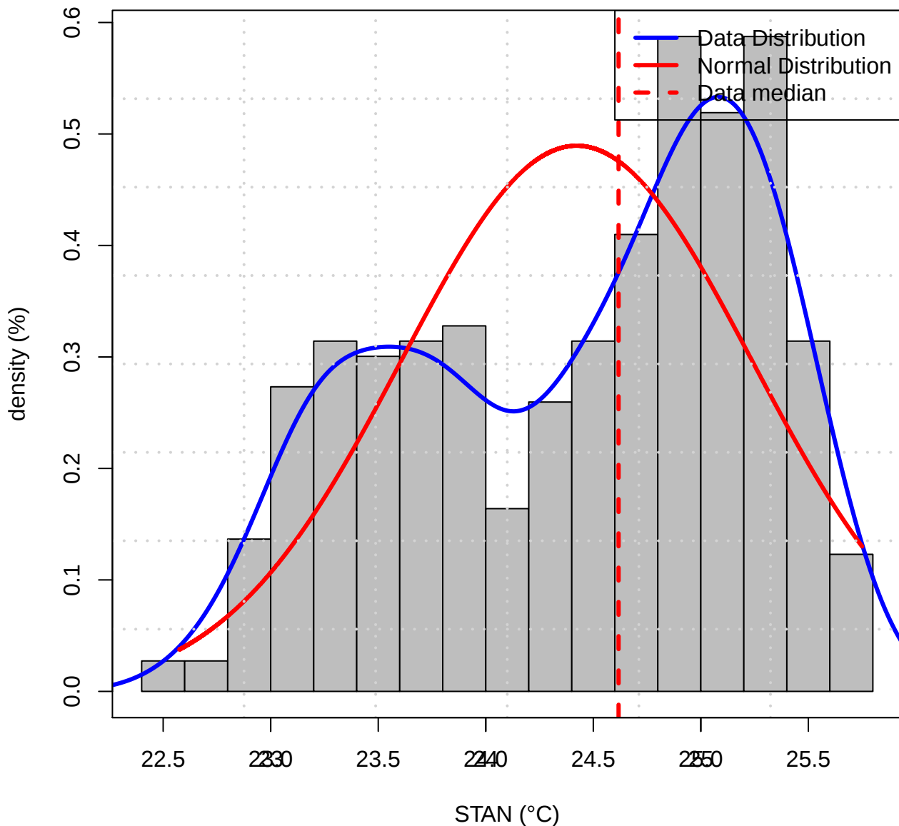
Histogram of Data distribution (TASMIN of STAN)
