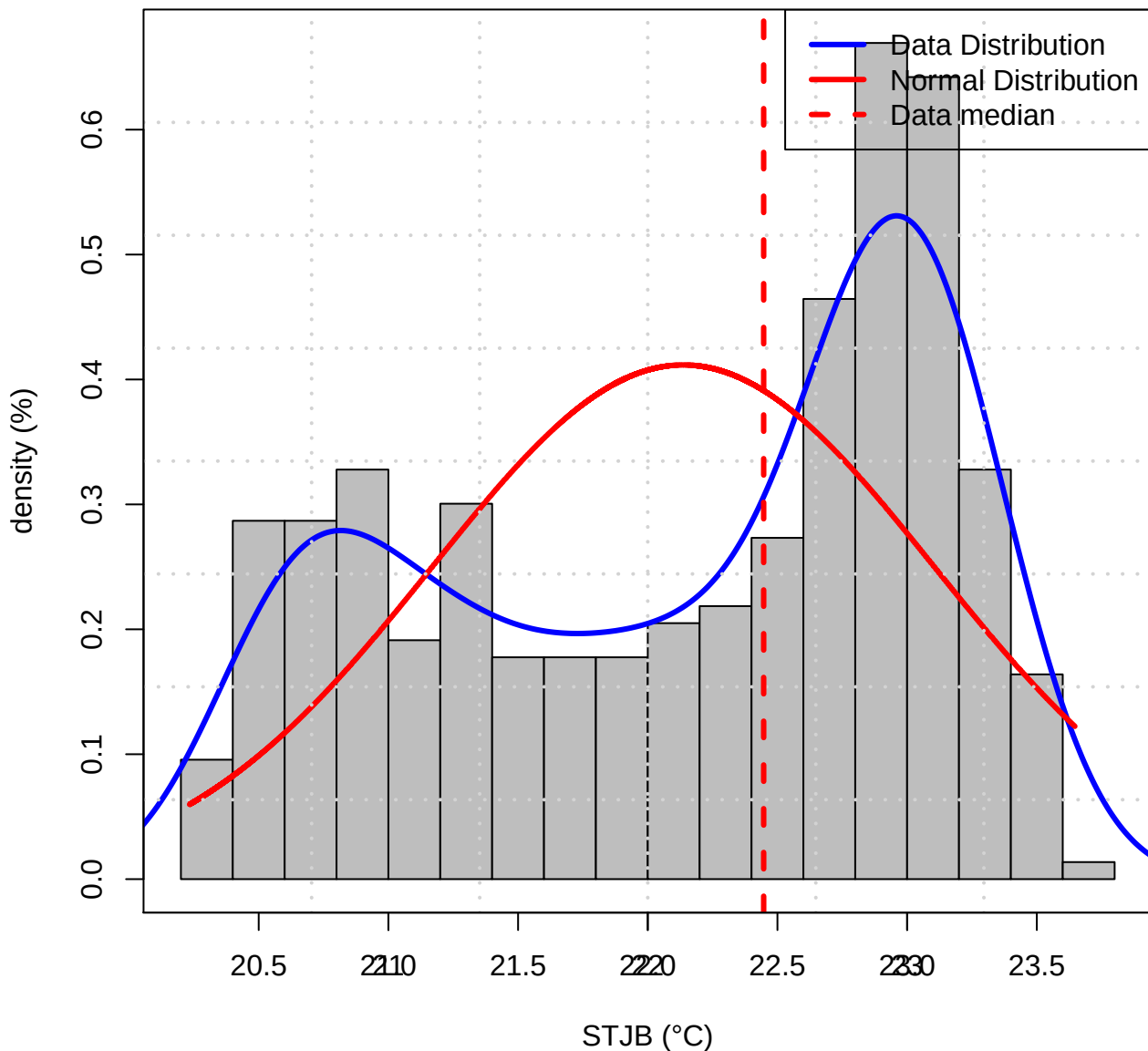
Histogram of Data distribution (TASMIN of STJB)
