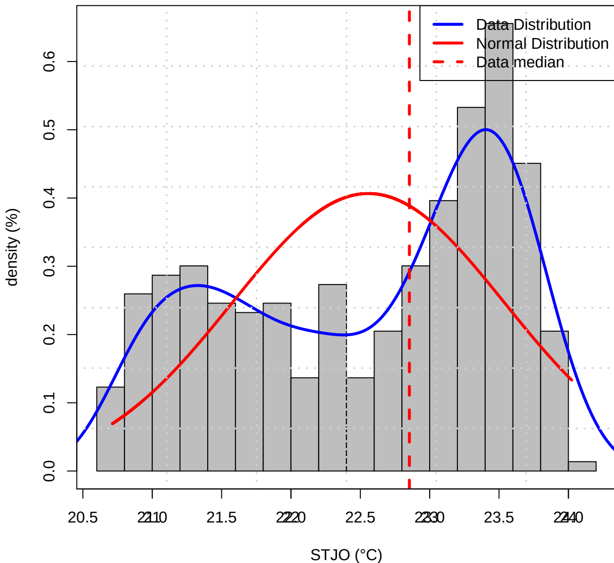
Histogram of Data distribution (TASMIN of STJO)
