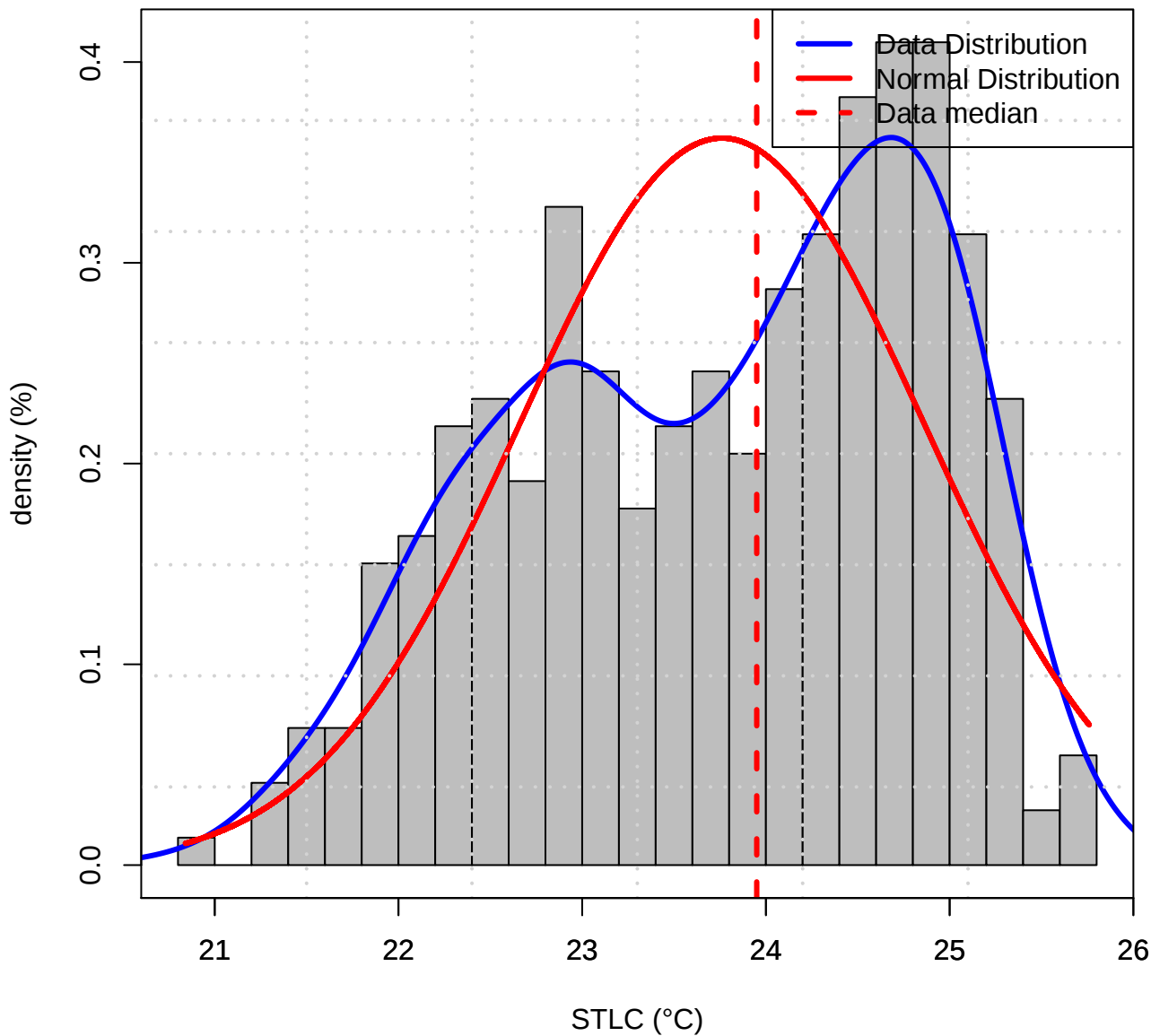
Histogram of Data distribution (TASMIN of STLC)
