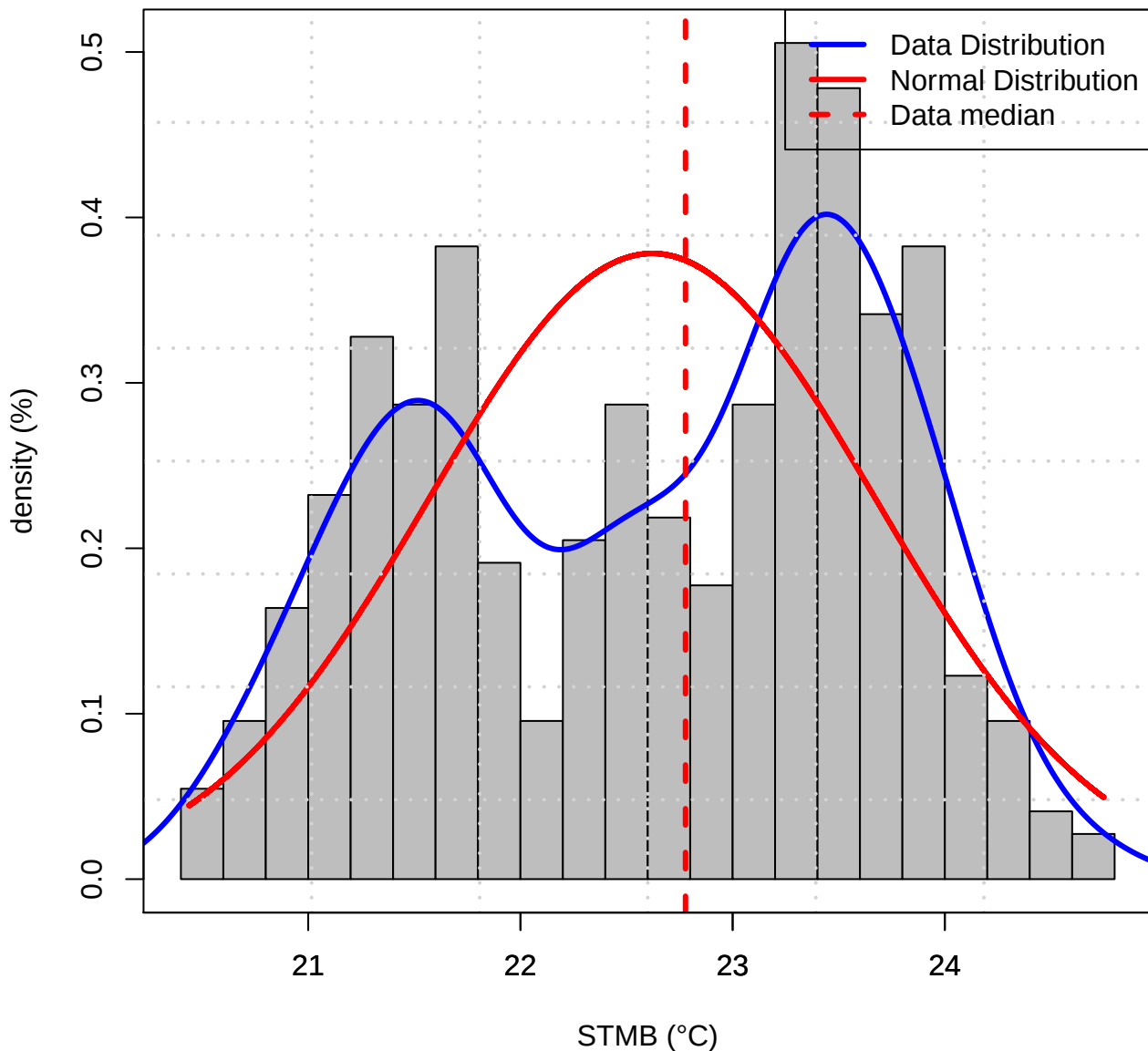
Histogram of Data distribution (TASMIN of STMB)
