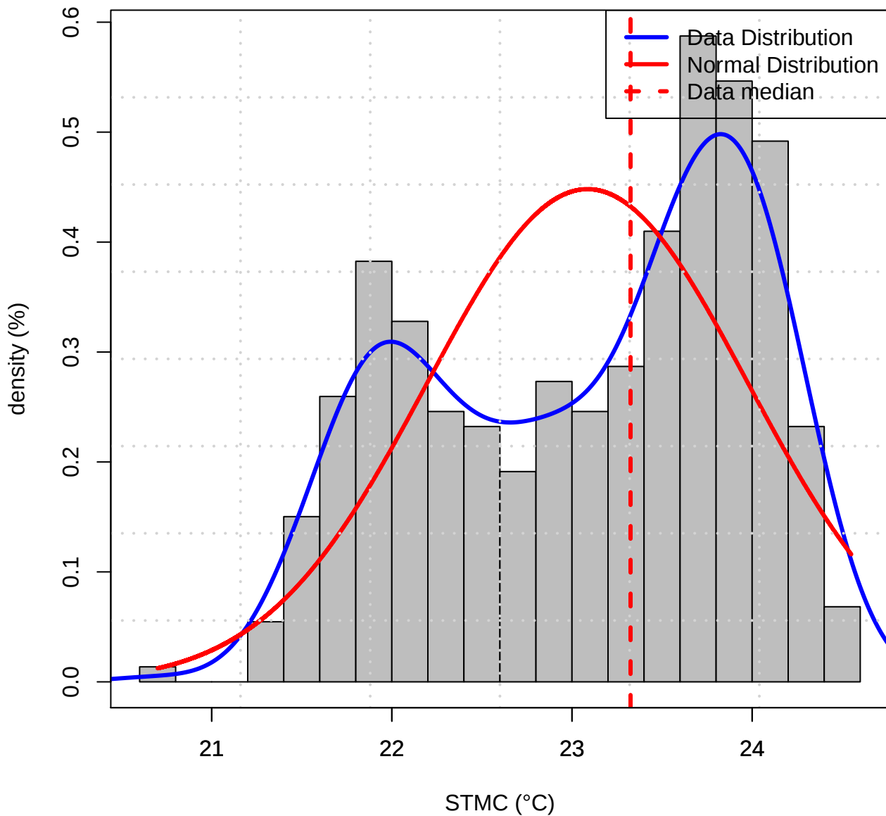
Histogram of Data distribution (TASMIN of STMC)
