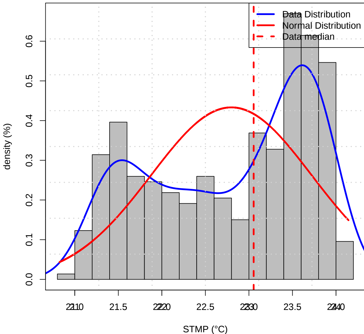
Histogram of Data distribution (TASMIN of STMP)
